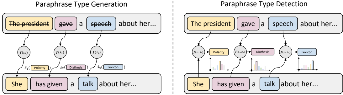
Figure 2: Paraphrase Type Generation (left) and Paraphrase Type Detection (right) with model f , reference segments s_1, s_2, s_3 and candidate segments \tilde{s}_1, \tilde{s}_2, \tilde{s}_3 .
