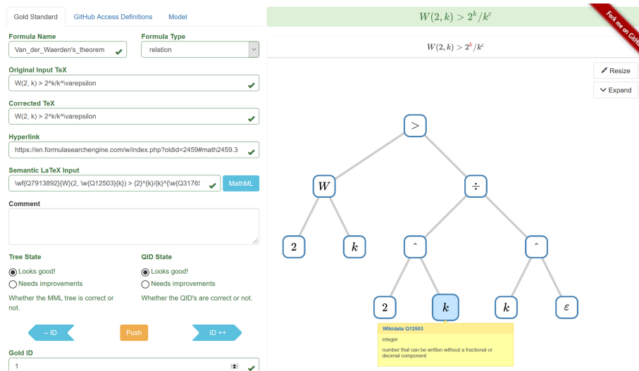
Figure 5: Graphical User Interface of MathMLben providing several TeX input fields (left) and a mathematical expression tree rendered by the VMEXT visualization tool (right) [22].
