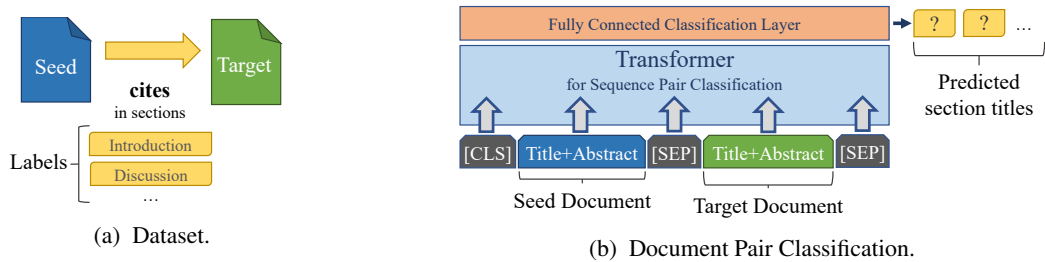
Figure 2: We use the section titles from citations as labels for document pairs. The sections define the aspects of the similarity. A Transformer model with titles and abstracts as input is used for classification.
