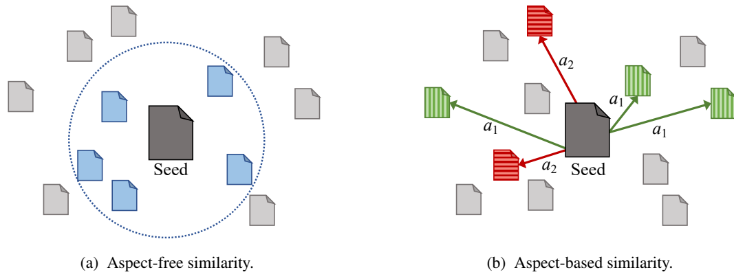
Figure 1: Most RS rely on similarity measures between a seed and the k most similar target documents (a). This neglects the aspects which make two or more documents similar. In aspect-based document similarity (b), documents are related according to the inner aspects connecting them ( a_1 or a_2 ).
